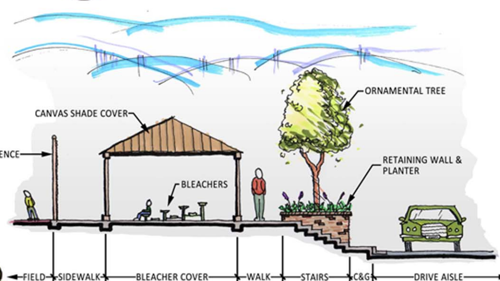
Bleacher Pad and Driveway - SECTION VIEW
